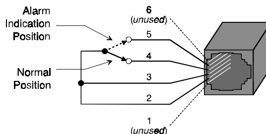
Figure 6 – Alarm (6 Position Modular Jack)
