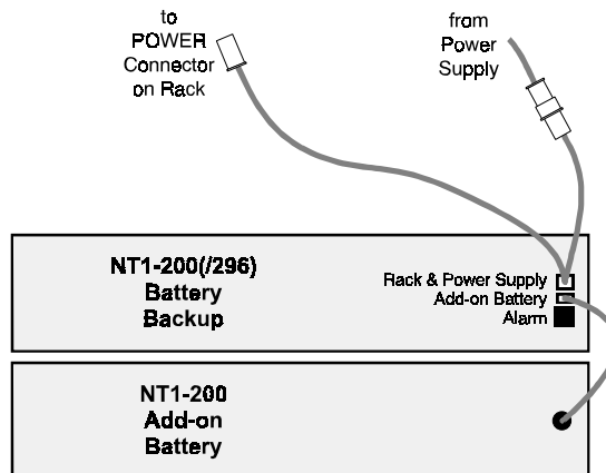
Figure 5 – Battery Connections
