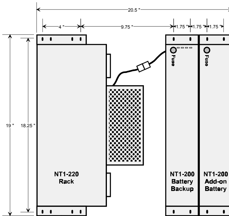
Figure 4 – Wall Mounting
