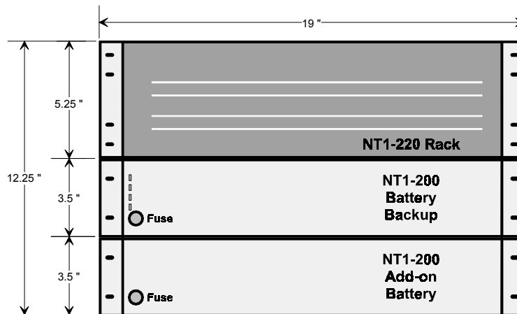
Figure 2 – Rack Mounting
